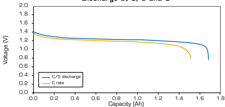
Discharge at C/5 and C
